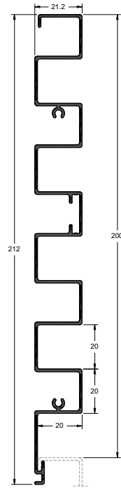
WD-2020 Cladding profile
