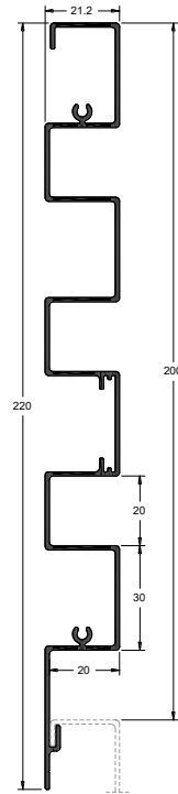
WD_2030 Cladding profile
