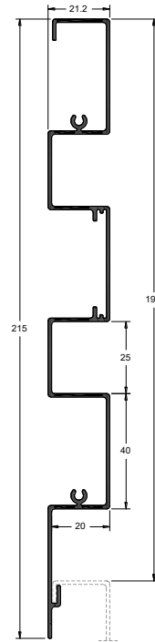
WD_2040 Cladding profile
