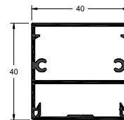
WD-4040 Decorative Profile
