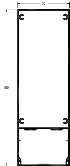
WD-1550 Decorative Profile
