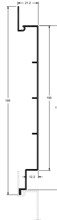
PF070-015 Cladding profile
