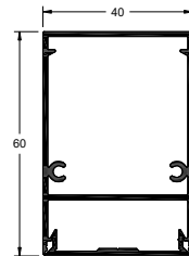
WD-6040 Decorative Profile
