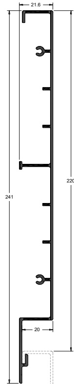
WD-2001 Cladding profile
