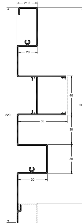
WD_2050 Cladding profile
